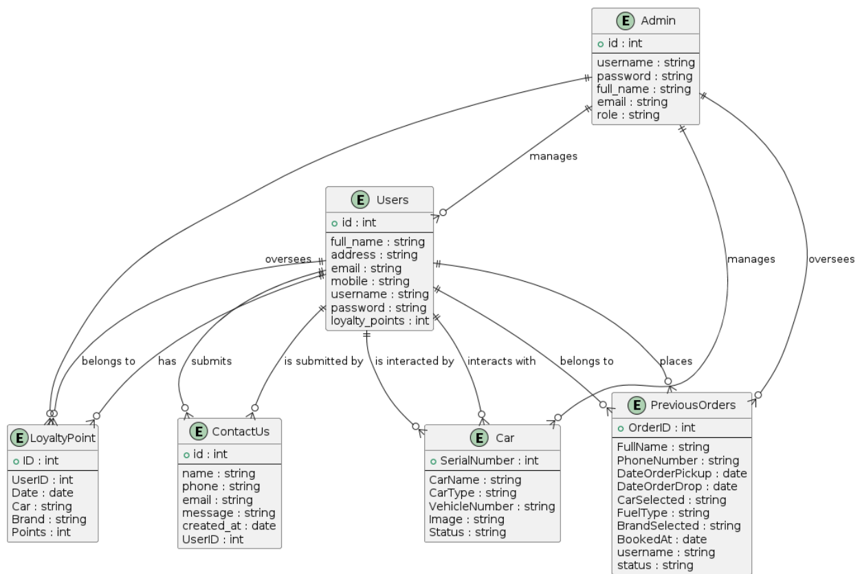
Figure 13 ERD
